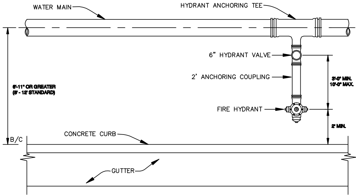
NORMAL HYDRANT SETTING PLAN VIEW
